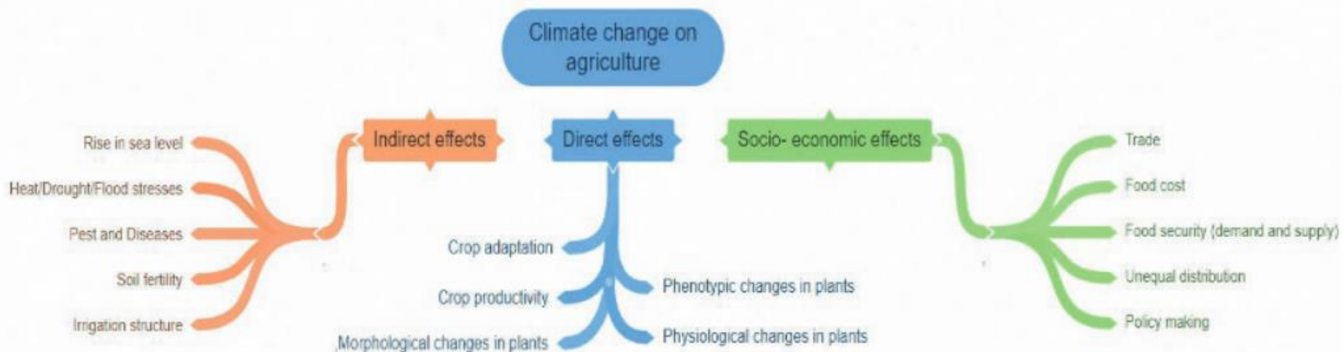
Figure 3. Direct, indirect and socio-economic effects of climate change on agriculture (Raza et al. , 2019)
