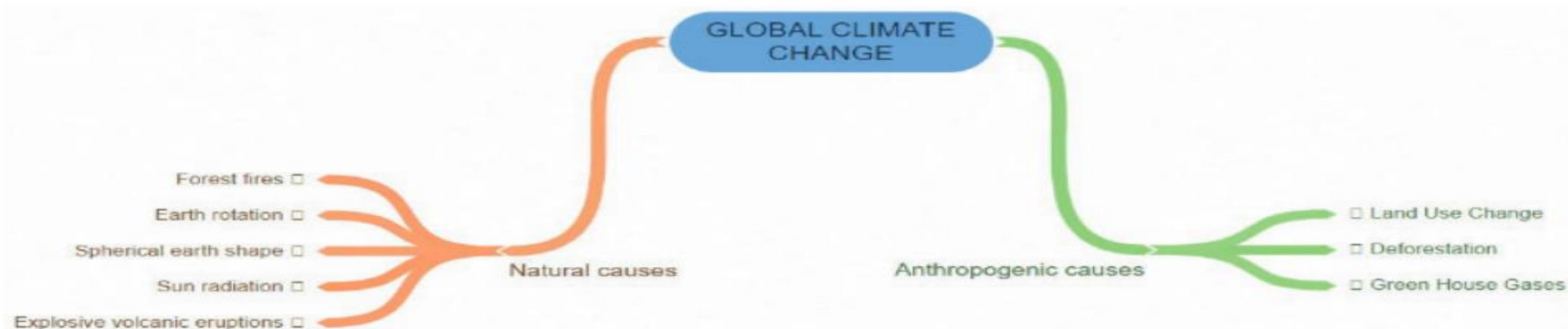
Figure 2. Causes of global climate change (Elmassah & Omran, 2014)
