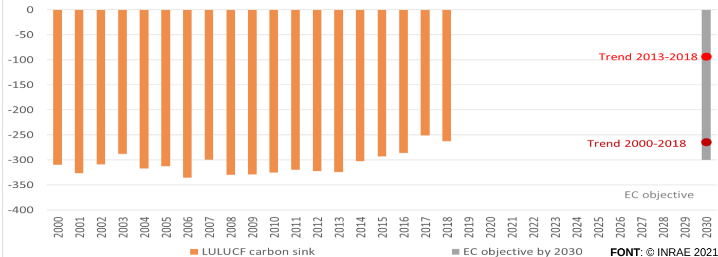
EU-27 carbon sink of the LULUCF sector (MtCO 2 eq)
